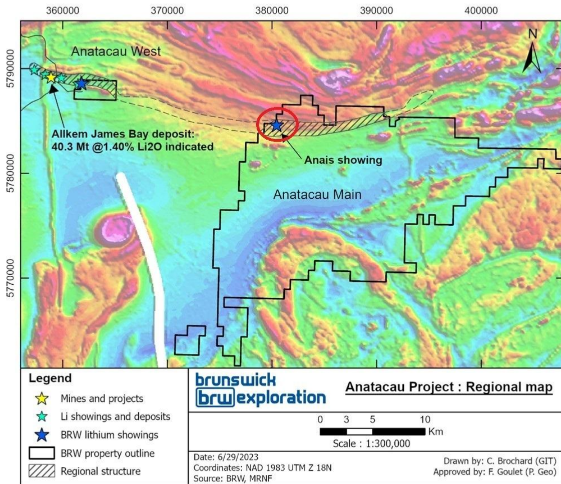
Regional Total Field Magnetic Map of the Anatacau West and Main Projects
